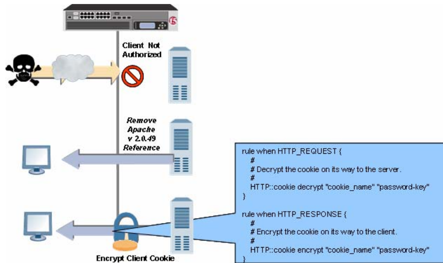
Encrypt/decrypt cookies
